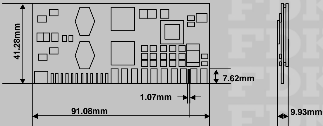
Sip Type(Isolation) High Density DC-DC Converter
