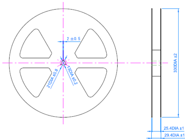
Figure 7-6 Reel dimensions
