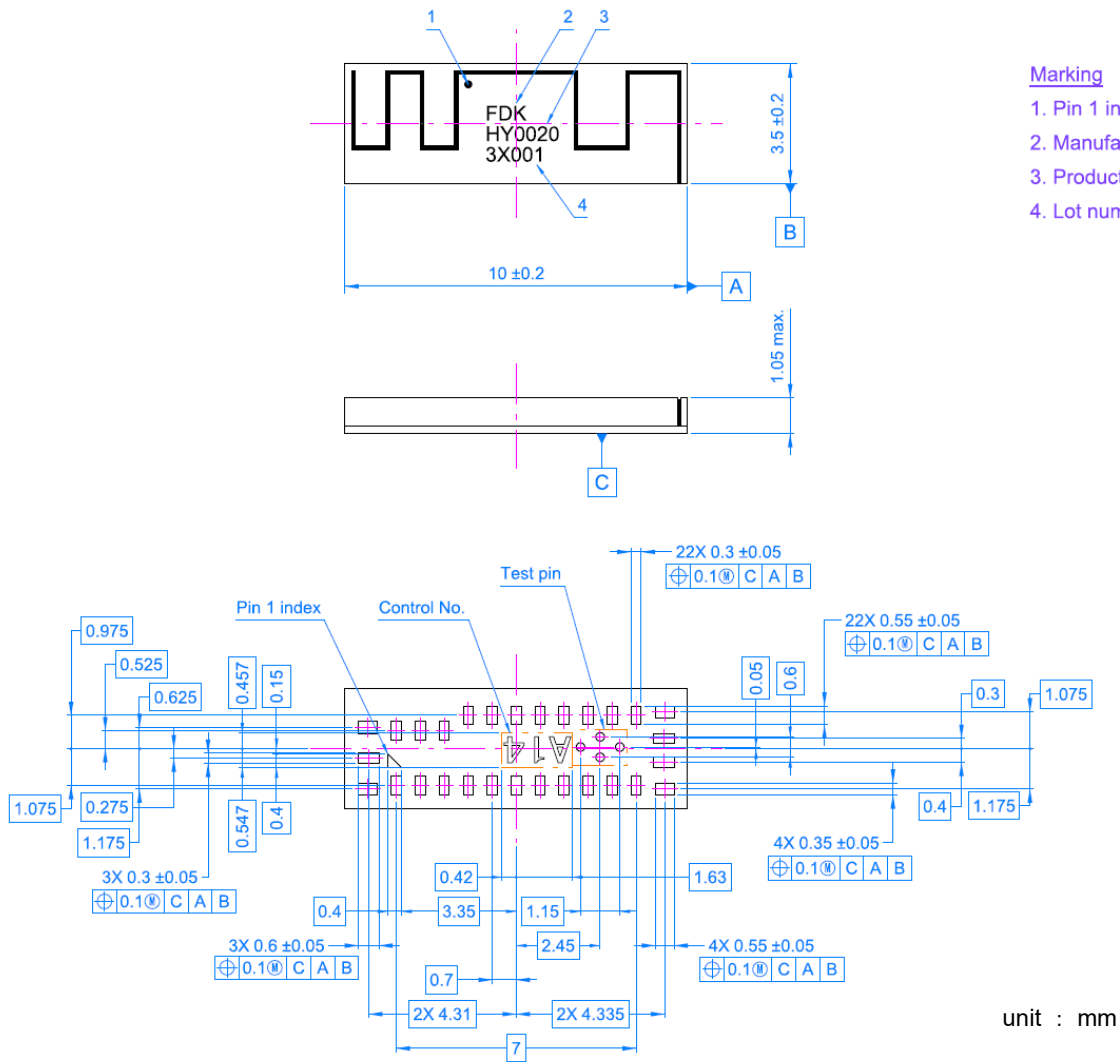
Figure 2-1 Outline
