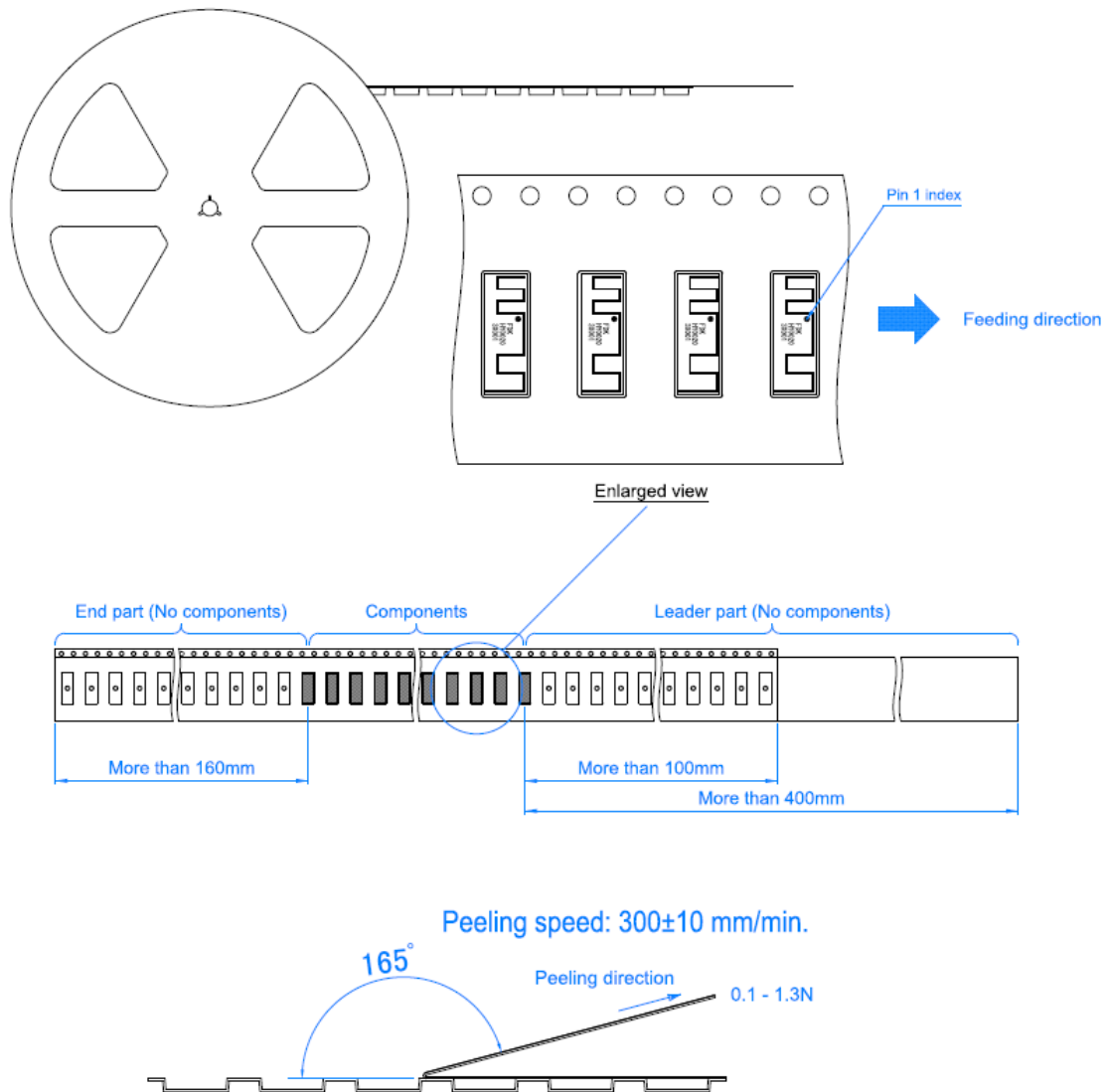
Figure 7-4 Tape specifications
