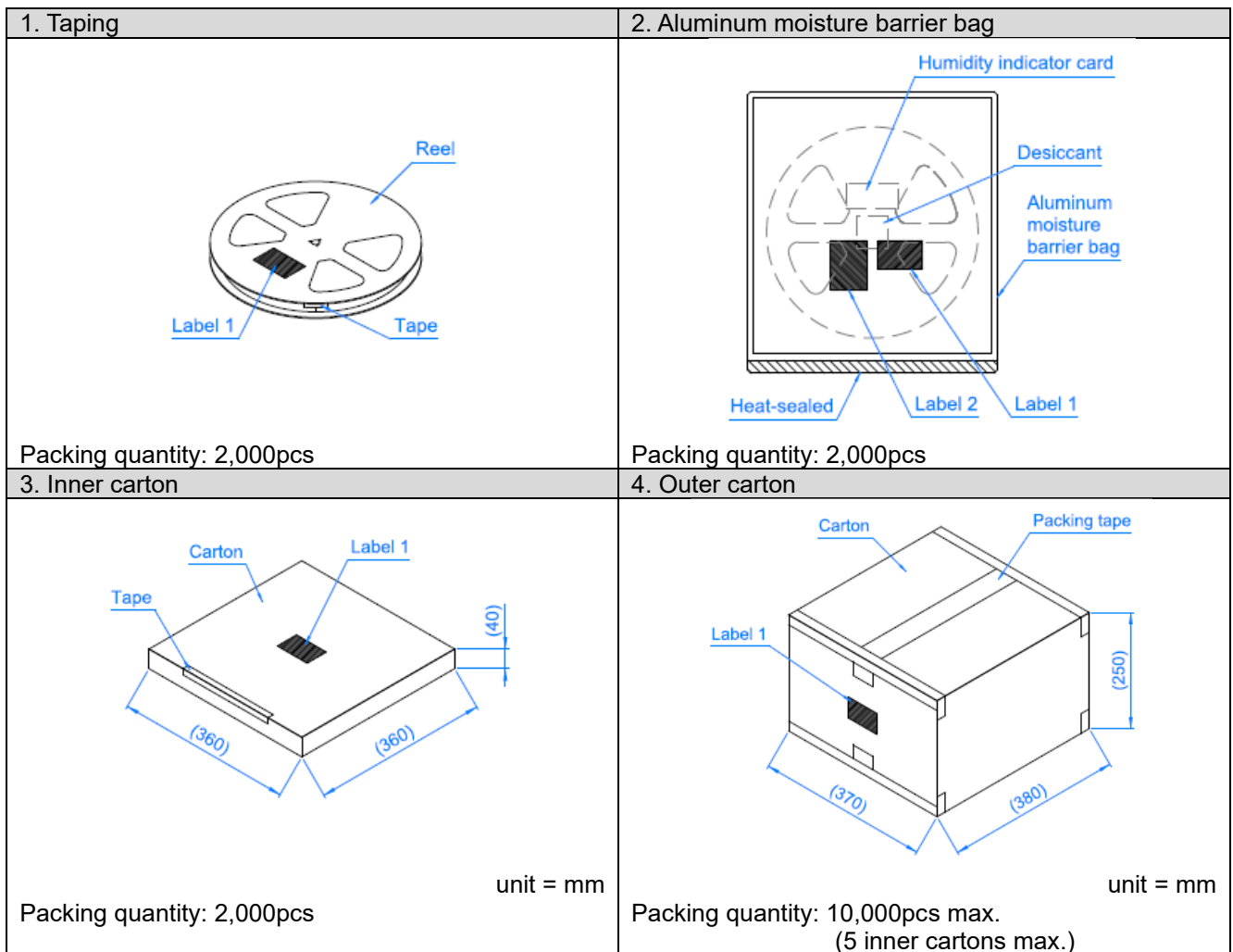
Figure 7-1 Packaging style
