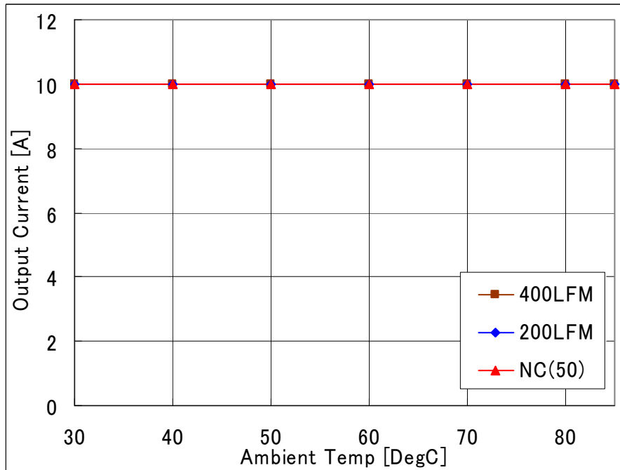
Fig-2.5V-1: Available load current vs. ambient temperature and airflow rates for V_{out}=2.5V with V_{in}=12.0V . Maximum component temperature \leq 120^{\circ}C
