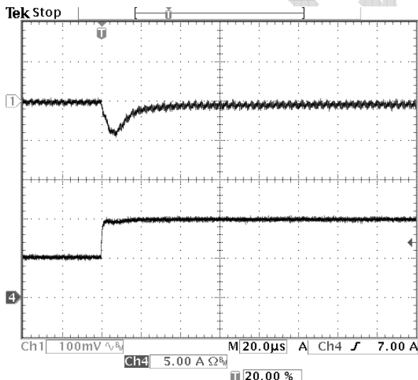
Fig-1.0V-6: Output voltage response for V_{out}=1.0V to positive load current step-change from 5A to 10A with slew rate of 5A/\mu s at V_{in}=12.0V . C_o=47\mu F \times 2 ceramic. Top trace: output voltage (100mV/div.) Bottom trace: load current (5A/div.) Time scale: 20μs/div.
