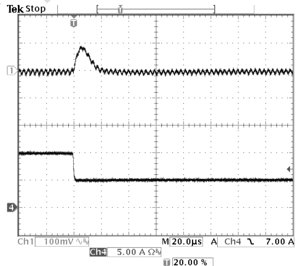
Fig-2.5V-7: Output voltage response for V_{out}=2.5V to positive load current step-change from 10A to 5A with slew rate of -5A/\mu s at V_{in}=12.0V . C_o=47\mu F \times 2 ceramic. Top trace: output voltage (100mV/div.) Bottom trace: load current (5A/div.) Time scale: 20\mu s /div.
