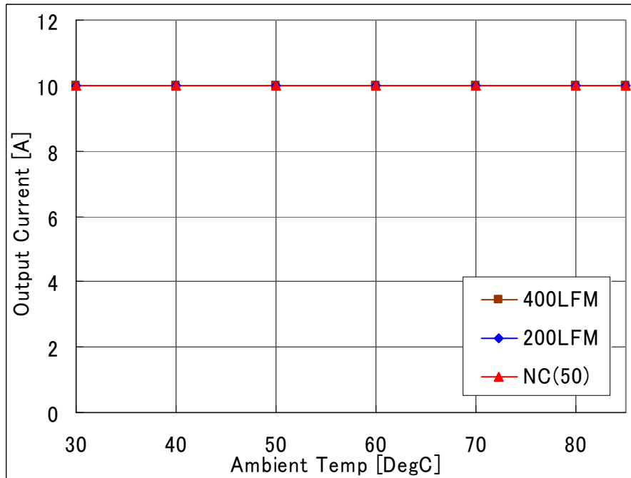
Fig-1.5V-1: Available load current vs. ambient temperature and airflow rates for Vout=1.5V with Vin=12.0V. Maximum component temperature \leq 120^{\circ}\text{C}
