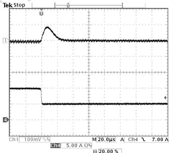
Fig-1.0V-7: Output voltage response for V_{out}=1.0V to positive load current step-change from 10A to 5A with slew rate of -5A/\mu s at V_{in}=12.0V . C_o=47\mu F \times 2 ceramic. Top trace: output voltage (100mV/div.) Bottom trace: load current (5A/div.) Time scale: 20μs/div.
