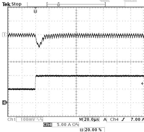
Fig-3.3V-6: Output voltage response for V_{out}=3.3V to positive load current step-change from 5A to 10A with slew rate of 5A/\mu s at V_{in}=12.0V . C_o=47\mu F \times 2 ceramic. Top trace: output voltage (100mV/div.) Bottom trace: load current (5A/div.) Time scale: 20μs/div.
