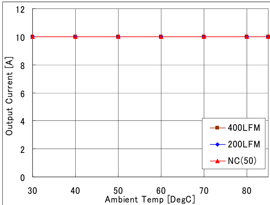
Fig-2.0V-1: Available load current vs. ambient temperature and airflow rates for V_{out}=2.0V with V_{in}=12.0V . Maximum component temperature \leq 120^{\circ}C
