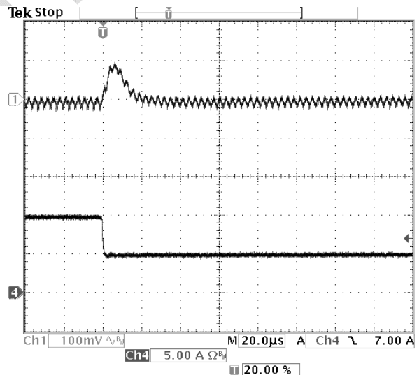
Fig-3.3V-7: Output voltage response for V_{out}=3.3V to positive load current step-change from 10A to 5A with slew rate of -5A/\mu s at V_{in}=12.0V . C_o=47\mu F \times 2 ceramic. Top trace: output voltage (100mV/div.) Bottom trace: load current (5A/div.) Time scale: 20μs/div.
