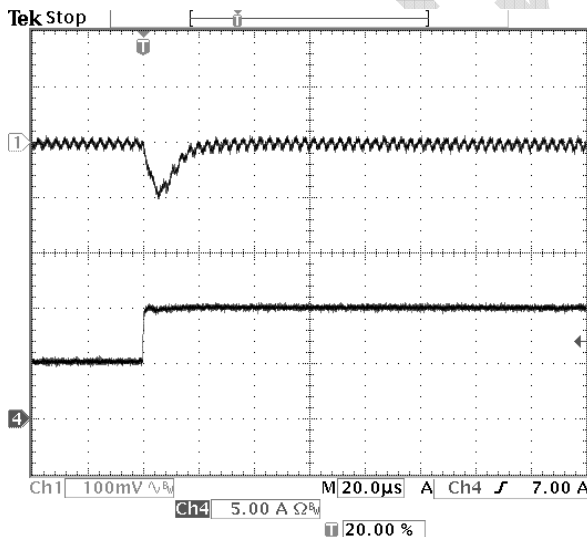
Fig-2.5V-6: Output voltage response for V_{out}=2.5V to positive load current step-change from 5A to 10A with slew rate of 5A/\mu s at V_{in}=12.0V . C_o=47\mu F \times 2 ceramic. Top trace: output voltage (100mV/div.) Bottom trace: load current (5A/div.) Time scale: 20\mu s /div.
