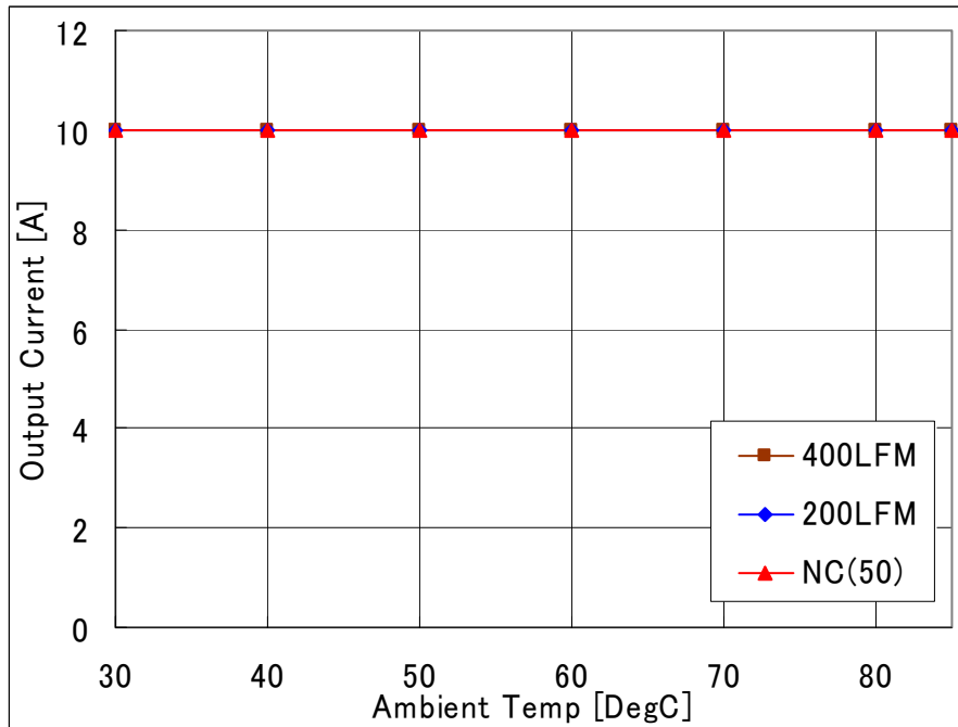
Fig-1.8V-1: Available load current vs. ambient temperature and airflow rates for V_{out}=1.8V with V_{in}=12.0V . Maximum component temperature \leq 120^{\circ}C
