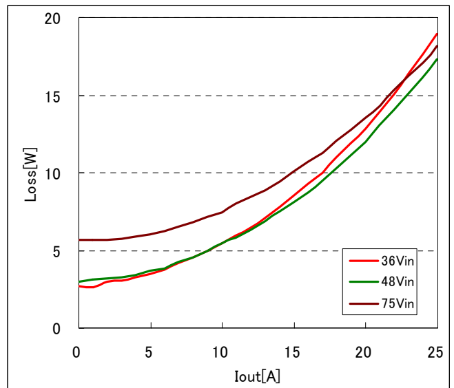
Fig.5.0V-3: Power Loss vs. load current and input voltage for converter mounted horizontally with airflow from pin 3 to pin 1 at a rate of 300LFM (1.5m/s) and Ta=25°C.
