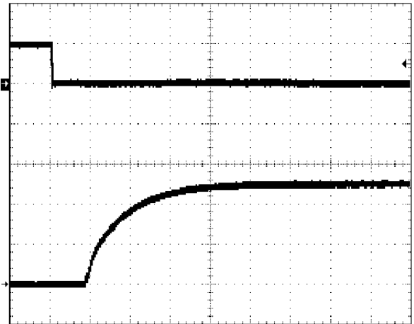
Fig.5.0V-5: Turn-on transient at full rated load current (resistive) plus 10,000 \mu F at Vin=48V, triggered via ON/OFF pin. Top trace: ON/OFF signal (10V/div). Bottom trace: output voltage (2V/div). Time scale: 5ms/div
