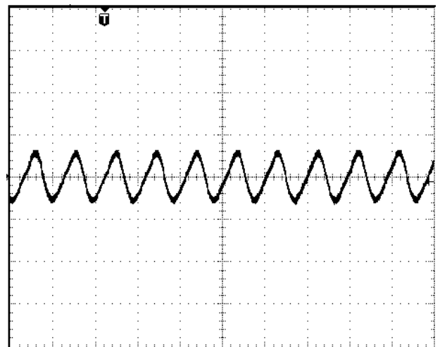
Fig.5.0V-10: Input reflected ripple current, I_c (200mA/div), measured through 10\mu\text{H} at the source at full rated load current and V_{in}=48\text{V} . Time scale: 2\mu\text{s}/\text{div} .
