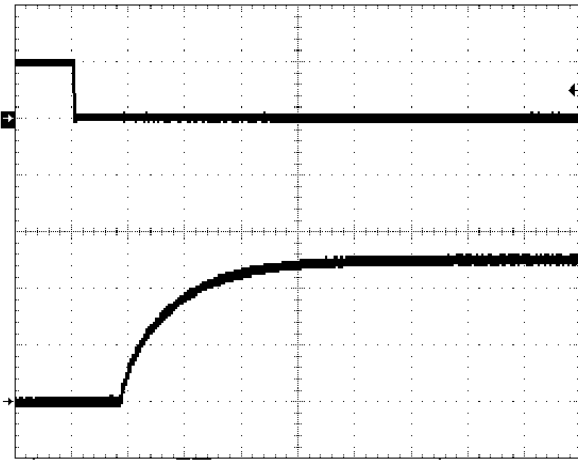
Fig.5.0V-4: Turn-on transient at full rated load current (resistive) with 10 \mu F tantalum + 1 \mu F ceramic capacitor at Vin=48V, triggered via ON/OFF pin. Top trace: ON/OFF signal (10V/div). Bottom trace: output voltage (2V/div). Time scale: 5ms/div
