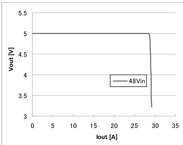
Fig.5.0V-11: Output voltage vs. load current showing current limit point and converter shutdown point. ( V_{in} = 48\text{V} )
