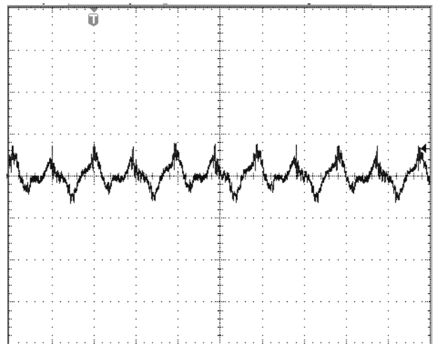
Fig.5.0V-7: Output voltage ripple (50mV/div) at full rated load current into a resistive load with Co=10 \mu F tantalum + 1 \mu F ceramic and Vin=48V. Time scale: 2 \mu s/div
