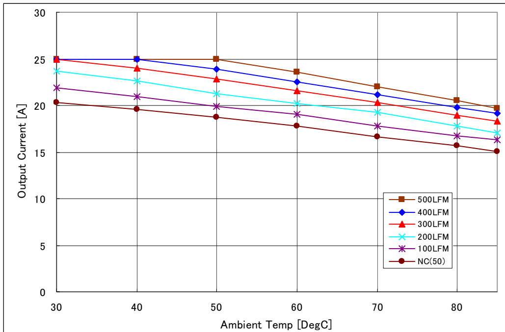
Fig.5.0V-1: Available load current vs. ambient temperature and airflow rates for Vin=48V. Maximum component temperature \leq 125^{\circ}\text{C}
