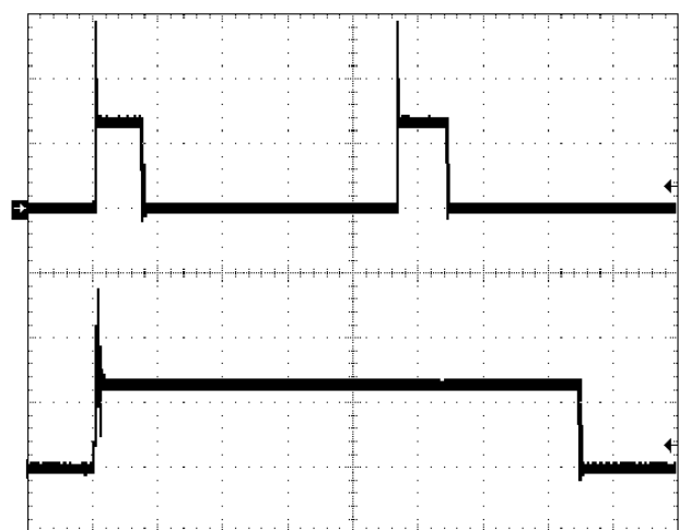
Fig.5.0V-12: Load current (top trace, 20A/div, 50ms/div) into a 10\text{m}\Omega short circuit during restart, at V_{in} = 48\text{V} . Bottom trace (20A/div, 1ms/div) is an expansion of the top trace.
