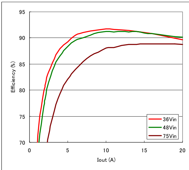
Fig.5.0V-2: Efficiency vs. load current and input voltage for converter mounted horizontally with airflow from pin 3 to pin 1 at a rate of 300LFM (1.5m/s) and Ta=25°C.
