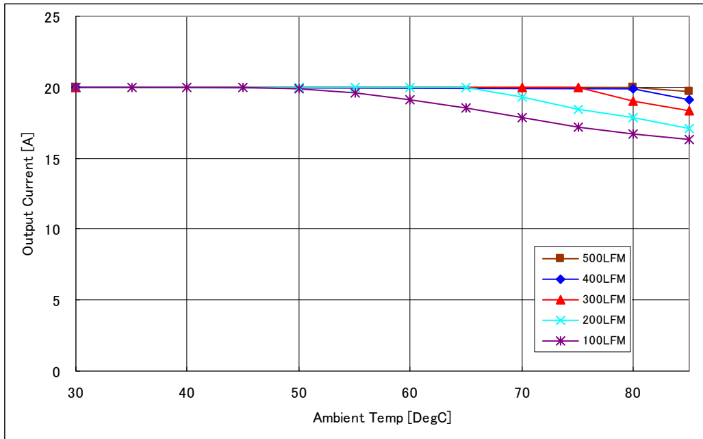
Fig.5.0V-1: Available load current vs. ambient temperature and airflow rates for Vin=48V. Maximum component temperature \leq 125^{\circ}\text{C}
