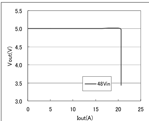
Fig.5.0V-11: Output voltage vs. load current showing current limit point and converter shutdown point. ( V_{in} = 48\text{V} )
